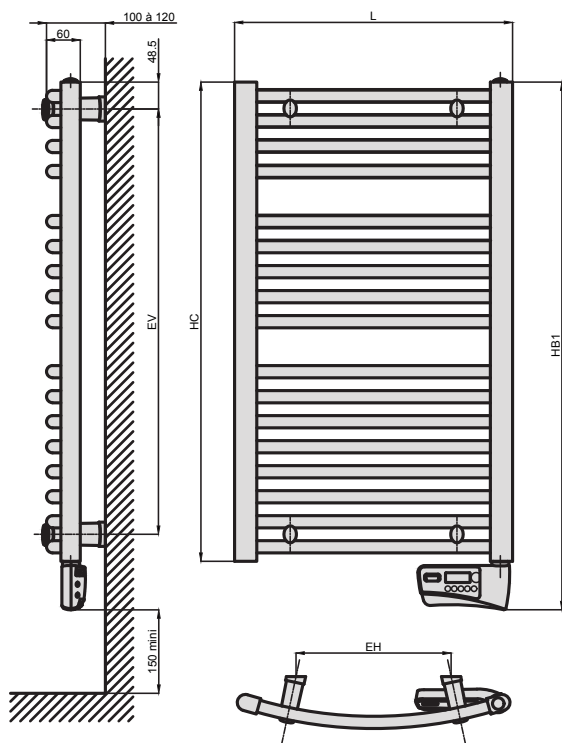
VERSION ELECTRIQUE standard
